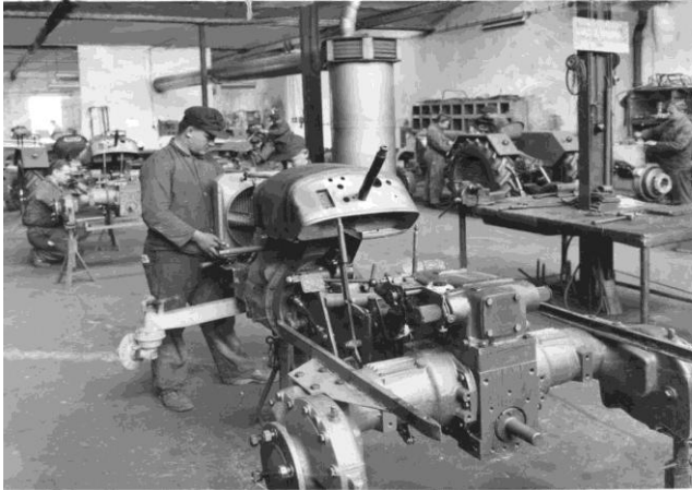
Wesseler Schlepper-Montage
